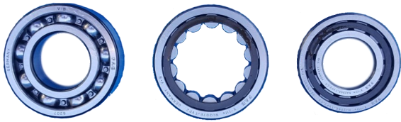
Main Case Bearings-- 6207, NJ207E.TVP2, NU206E.TVP2
